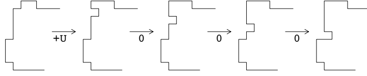
FIG. 7. Creation and motion of the hole at cost 0.
