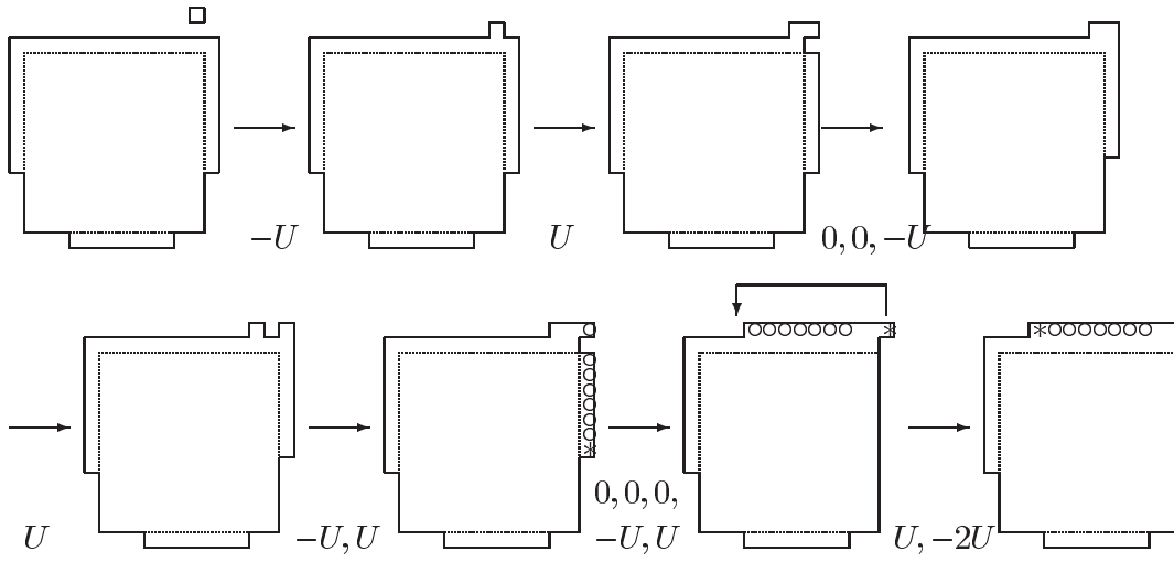
Fig. 11. An example of a path from \mathcal{C}^B to \blacksquare .
