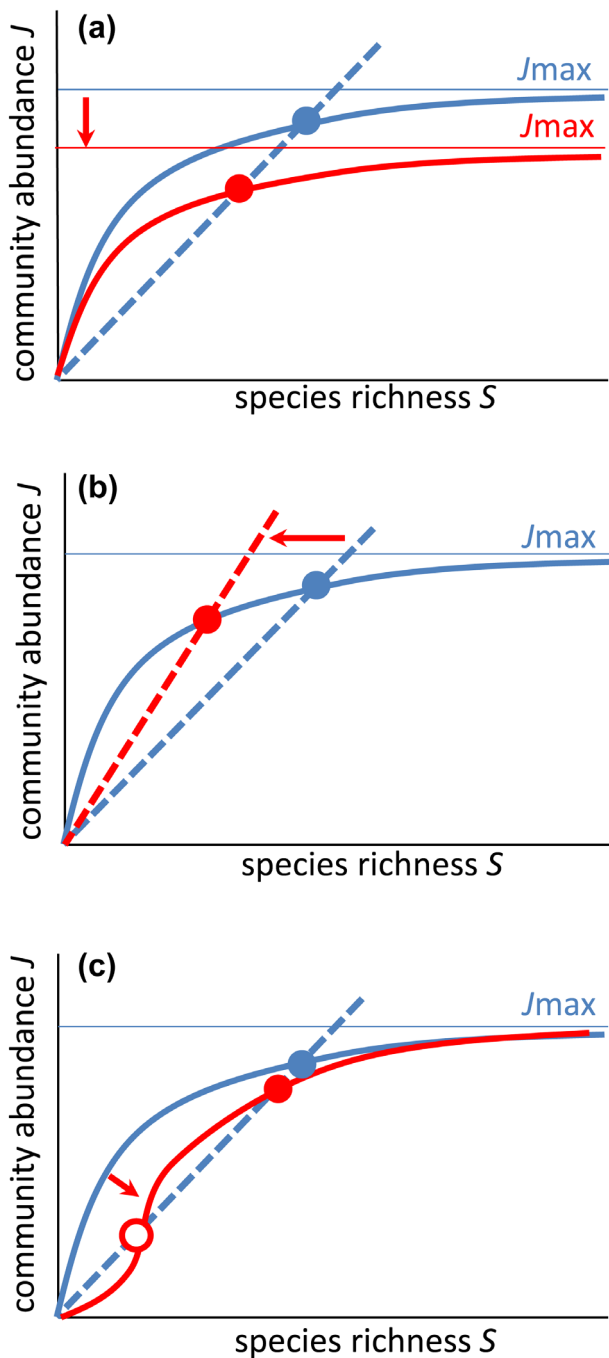
Figure 4. Humans may modify equilibrium diversity by several conceptually distinct ways (red arrows). Dashed curves indicate S -nullclines, bold solid lines are J -nullclines, filled circles are stable equilibria, blue refers to the pre-Anthropocene condition and red to the anthropogenic modifications. (a) Reduction of resource supply by appropriation of primary productivity or habitat degradation leads to lowering maximum community abundance J_{\max} (which is given by total potential energy flow through the community E divided by mean metabolic rate B ; J_{\max} = E/B ). Due to non-linear J -nullclines, this leads to non-linear effects on the shifts of diversity equilibria. (b) Alternatively, humans may affect extinction or origination rates (Fig. 1c–d), increasing the mean population abundance
