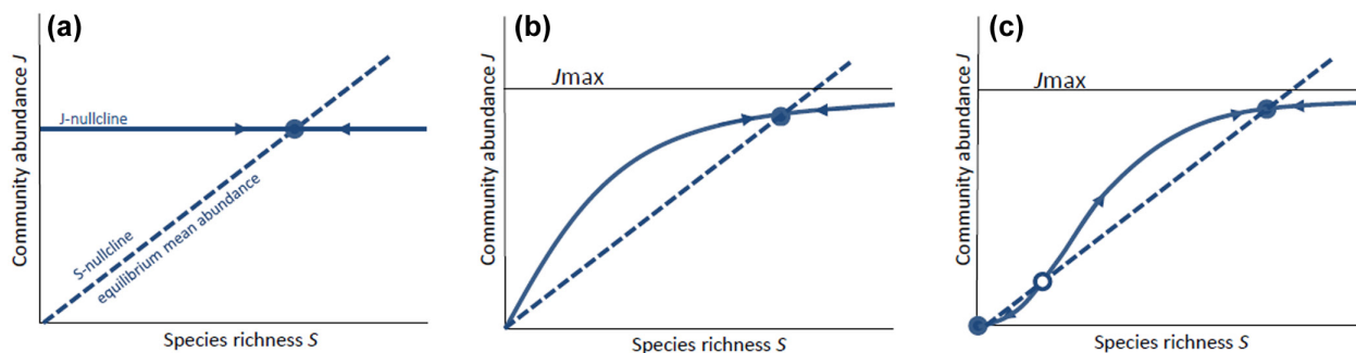
Figure 2. Graphical analysis of ETDB showing how diversity equilibria depend on the dynamics of both species richness ( S ) and total community abundance ( J ). Due to the population size-dependence of the rates of species origination and extinction, ETDB predicts that, for a given species-abundance distribution (SAD), there exists an equilibrium mean species abundance, \hat{N} , in which origination and extinction rates are balanced (Fig. 1). All potential diversity equilibria thus lie on an S -nullcline (dashed line) that delineates the values of S and J at which dS/dt=0 and whose slope corresponds to \hat{N} (i.e. J = \hat{N}S ). However, the realized equilibrium state also depends on J being in equilibrium, so equilibrium S and J must lie on the intersection (full circle) of the diagonal S -nullcline and a J -nullcline, which relates J to S when dJ/dt=0 (solid line/curve). Out-of-equilibrium communities follow near-vertical paths towards their J -nullclines and then the arrows along the J -nullcline towards stable equilibria (full circles). (a) In one extreme scenario, the J -nullcline is independent of S and so it is just a horizontal line. (b) However, a more realistic scenario is that increasing species richness increases a community's ability to utilize resources, so that the J -nullcline increases with S until it reaches its thermodynamic limit J_{\max} . In the extreme that species are entirely independent of each other (strict niche complementarity), the J -nullcline increases linearly with S until it reaches its limit. However, as some species share resources and compete, the J -nullcline generally exhibits little linearity and rather likely decelerates at higher S due to increasing competition. (c) The J -nullcline may be even more complex, e.g. sigmoidal, which can lead to two equilibrium points, one stable (full circle) and the other unstable (empty circle). Such a situation can emerge when facilitation dominates over some range in S , which accelerates the J -nullcline. Here, at low S , several species need to support each other in their resource utilization in order for the J -nullcline to be high enough for communities to obtain higher rates of origination than extinction. A loss of species below the unstable equilibrium leads to inevitable extinction of further species which is not compensated by origination.
