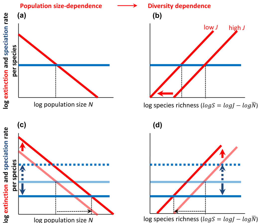
Figure 1. Overview of how biodiversity equilibria emerge and are influenced by anthropogenic changes. Here we deal with large-scale (regional) biodiversity in which biodiversity equilibrium is maintained by a balance of speciation and extinction with the contribution from colonization being negligible (Fig. 3 for the effects of colonization on local-scale dynamics). (a) Rates of speciation (blue lines) and extinction (red lines) are population size-dependent. For simplicity and with minimal loss of generality, we assume this population size-dependence can be approximated as power-laws, i.e. lines in log-log space. Additionally, we assume here that speciation rate is population size-independent (i.e. the slope of the power-law is zero), as this simplifies the figure without altering the general insights; the only condition of stable equilibrium is that the slope of the speciation function is higher than the slope of the extinction function and the lines intersect. This condition is expected to be near-universal, due to extinction rate decreasing substantially with population size, unlike speciation rate. Mean population size at equilibrium (corresponding to no net change of species richness) is determined by the intersection of the lines (vertical black line). (b) This population size-dependence translates into diversity dependence, since mean population size \bar{N} = J / S , where J is total community size (total number of individuals) and S is species richness. Increasing S at a given J thus implies lower \bar{N} and consequently increasing average per species extinction rate. A decrease in J (e.g. due to anthropogenic removal of resources, red arrow) decreases equilibrium species richness by temporarily decreasing \bar{N} and so increasing extinction rate until the new lower equilibrium is reached. (c) Equilibrium richness can also change due to an increase in the probability or level (intercept) of extinction (red arrow), e.g. due to increased populations fluctuations or direct population exploitation. Anthropogenic effects can also modify speciation rates, either towards lower (Rosenzweig 2001, blue solid arrow) or higher levels (Thomas 2017, blue dotted arrow, dotted horizontal line). Note that increased overall levels of extinction and/or decreased overall level of speciation increase the equilibrium \bar{N} (dashed black arrow). (d) These changes are reflected in the shift of equilibrium species richness. Anthropogenic changes in equilibrium richness are thus predicted to be associated with changes of equilibrium mean population size when humans affect per species extinction and speciation levels, whereas no changes in equilibrium mean population size are expected if reductions in equilibrium richness are driven only by decreases in J . Note that J itself can be affected by species richness, which can lead to more complex and non-linear equilibril dynamics (Fig. 2).
