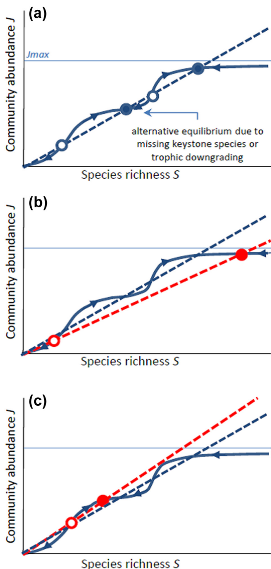
Figure 5. Schematic of the equilibrium theory of biodiversity dynamics applied to a hypothetical ecosystem or biome showing how human effects on extinction, origination and diversity's role in ecosystem functioning can create tipping points and affect the number and position of equilibria. Here we assume the J -nullcline (bold blue curves) is complex and reflects aggregate effect of species richness on the ability to utilize ecosystem resources and convert those resources into community abundance J . Dashed lines are S -nullclines determined by population size-dependencies of extinction and origination rates. (a) The hypothetical ecosystem/biome has two stable equilibria due to keystone species or trophic levels enhancing resource use or ecosystem functioning; declines in keystone species and trophic levels remove the second accelerating phase and thus the higher richness equilibrium. (b) Higher origination rates or reduced extinction rates (red dashed line) remove the intermediate stable richness equilibrium and increase the richness of the other stable equilibrium. (c) Lower origination rates or higher extinction rates (red dashed line) remove the higher stable richness equilibrium, as well as its basin of attraction (distance to the nearest unstable equilibrium), and thus the resilience of the system.
