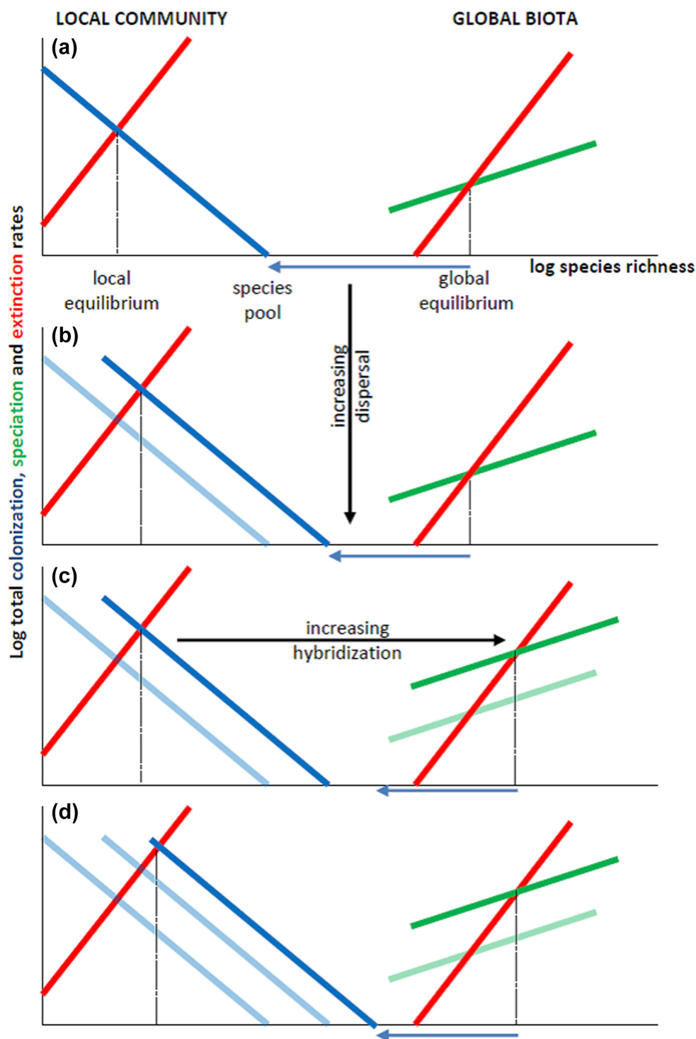
Figure 3. Effects of spreading of non-native species on local (left) and global (right) diversity equilibria (see the text for explanations). Here we assume that the diversity-dependent rates of speciation, colonization and extinction can be expressed as power-laws (lines in log-log space) and that the slopes of these lines (reflecting the strength of diversity dependency) are fixed, but that humans can affect their overall levels (intercepts). Note that in contrast to Fig. 1 where per-species rates are depicted, the lines here refer to total rates across all species. (a) Pre-Anthropocene situation, in which local equilibrium species richness is given by the balance of extinction (red) and colonization (blue), and colonization rate is determined by the effective size of the species pool, which represents a fraction (depicted by blue arrow) of global biodiversity richness, which is itself a result of extinction and speciation (green). (b) During the Anthropocene, increased movement of organisms across the planet have increased the fraction of global biodiversity available for local communities (shorter blue arrow), which increases colonization rate and thus local equilibrium richness. (c) Higher local species richness leads to new species combinations, increasing speciation rates (e.g. due to hybridization, or novel adaptations) and thus elevating global diversity. (d) This further elevates local equilibrium diversity due to further enriching species pools. These effects, however, may be only temporary, due to the gradual depletion of the pool of non-native colonizers.
